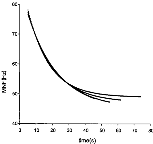
Figure 3: Comparison of the fitted curves of the original data (the longest) and the truncated data.
