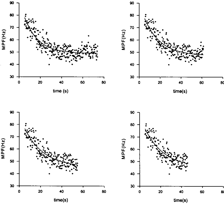
Figure 3: Comparison of the fitted curves of the original data (the longest) and the truncated data.
