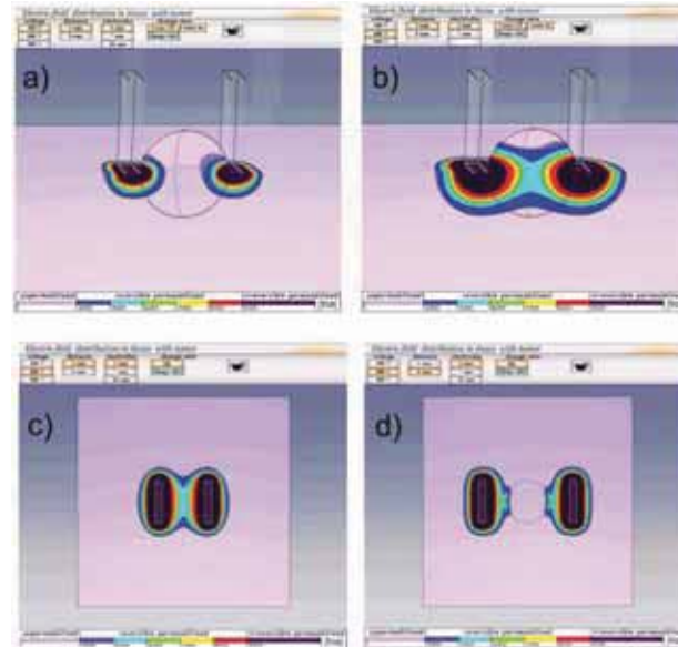
Figure 6. Electric field distribution inside the protruding tumor model for two different applied voltages on the electrodes: a) U = 300 V and b) U = 600 V. The electrodes are 4 mm wide and 4 mm apart in both cases. Electric field distribution inside the models for two distances between electrodes: c) d = 4 mm and d) d = 8 mm. The electrodes are 4 mm wide with the applied voltage U = 600 V in both cases.
